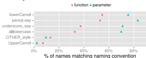
Figure 1: The percentage of function and parameter names from CRAN that matches the five naming conventions.
